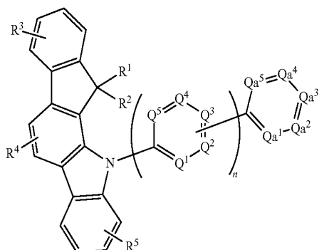
[Chemical Formula 5]
