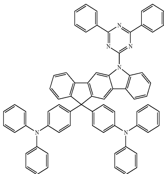
[Chemical Formula 22]
