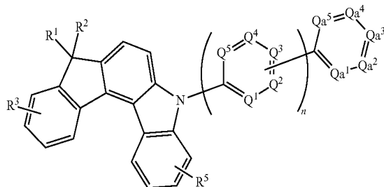
[Chemical Formula 9]
