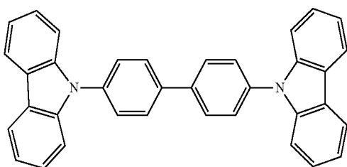
[Chemical Formula 35]
