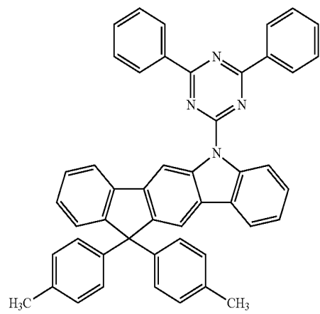
[Chemical Formula 13]
