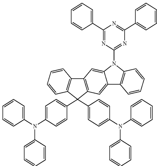
[Chemical Formula 22]
