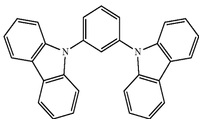
[Chemical Formula 36]
