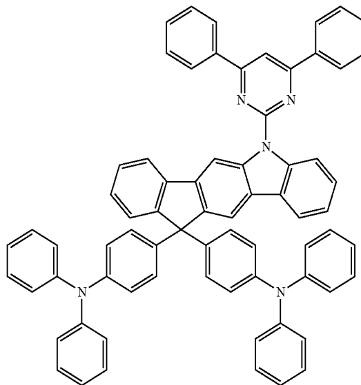
[Chemical Formula 24]
