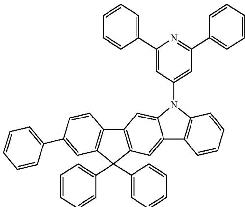
[Chemical Formula 17]
