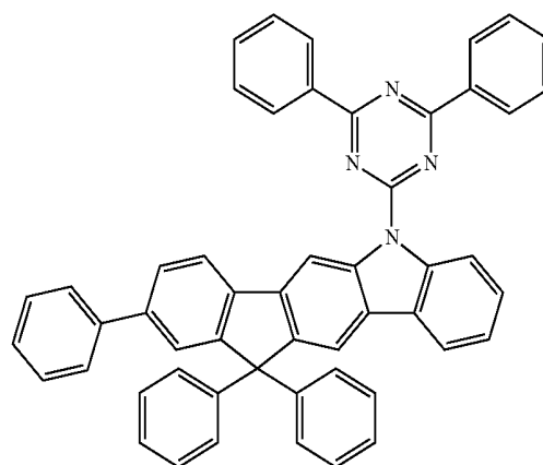
[Chemical Formula 16]
