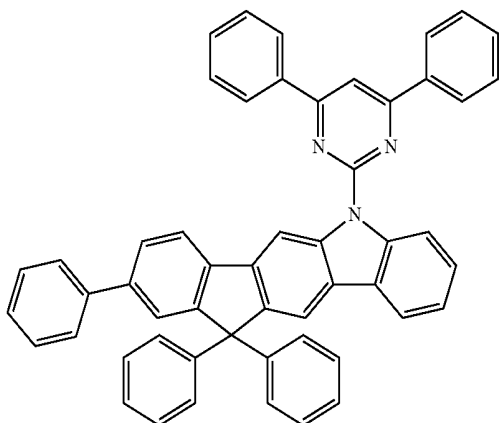
[Chemical Formula 18]
