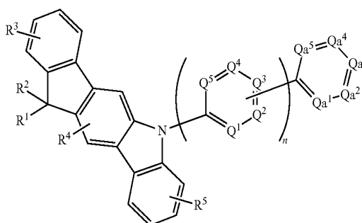
[Chemical Formula 4]
