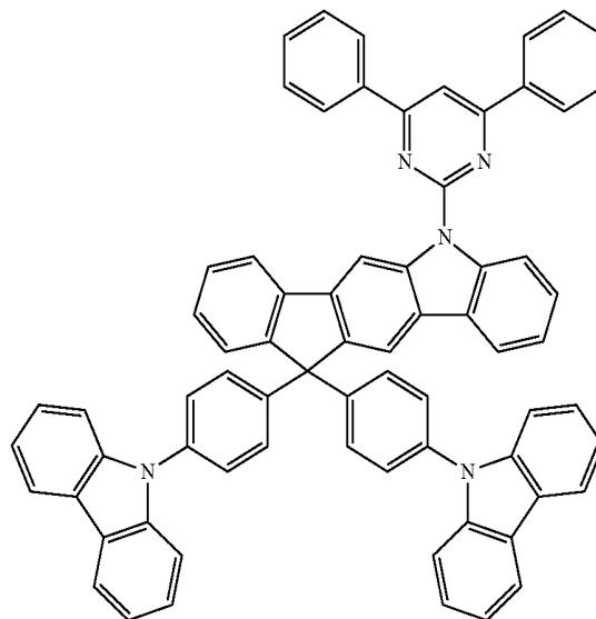
[Chemical Formula 21]
