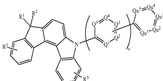
[Chemical Formula 8]
