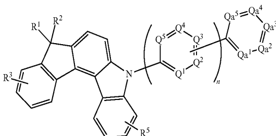
[Chemical Formula 8]
