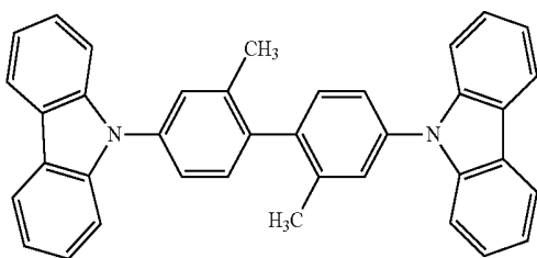
[Chemical Formula 37]
