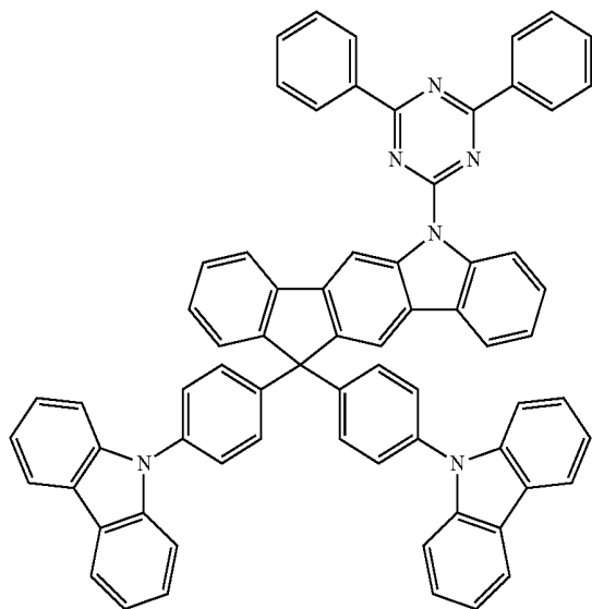
[Chemical Formula 20]
