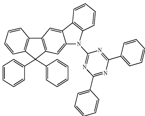
[Chemical Formula 25]
