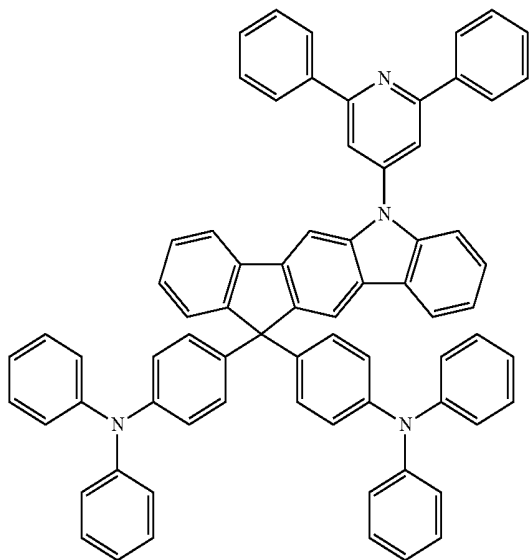
[Chemical Formula 24]
