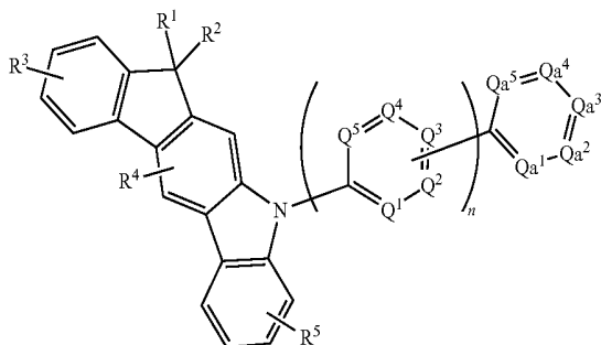
[Chemical Formula 6]
