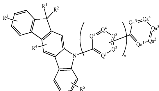
[Chemical Formula 6]
