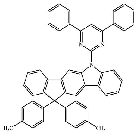
[Chemical Formula 15]
