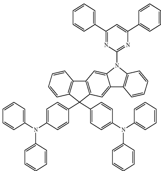
[Chemical Formula 25]
